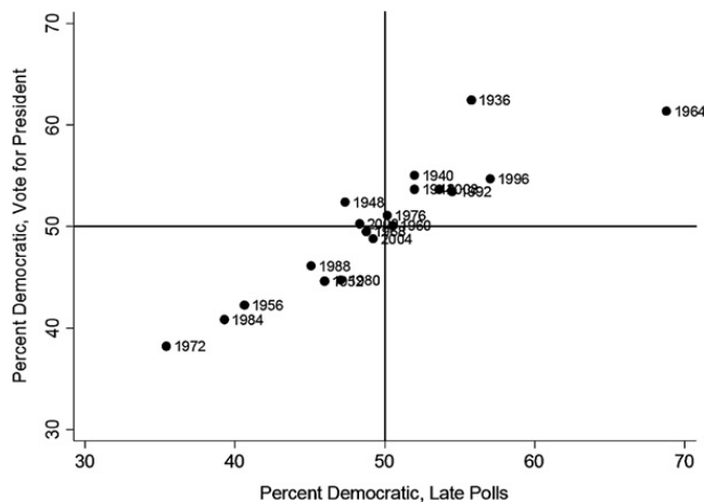
Fig. 3. Predicting the vote from the polls, 1936–2008.
