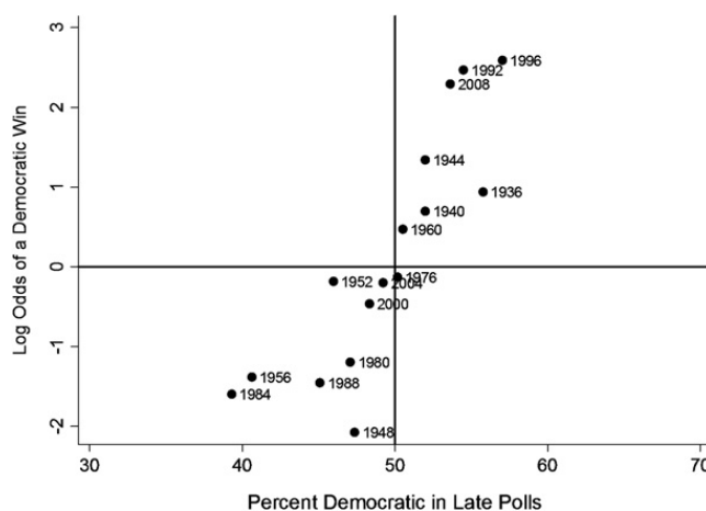
Fig. 4. Predicting the market prices from the polls, 1936–2008.
